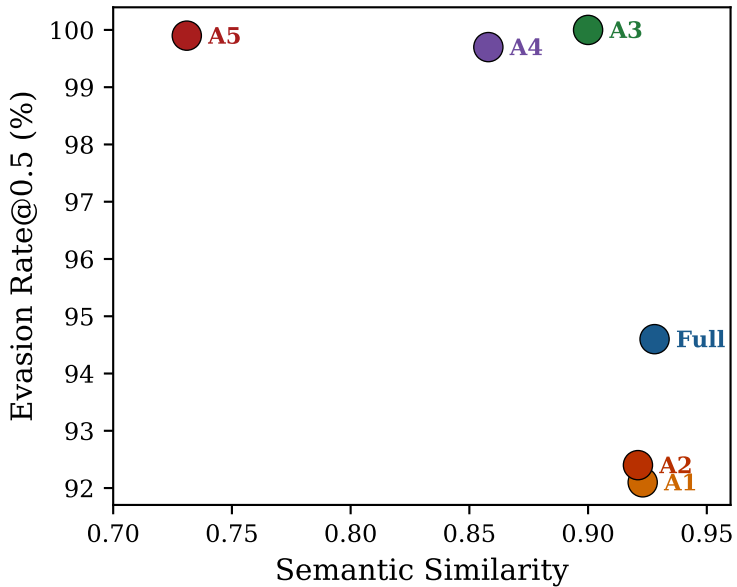
(a) Similarity vs Evasion ( \gamma=7.0 )
