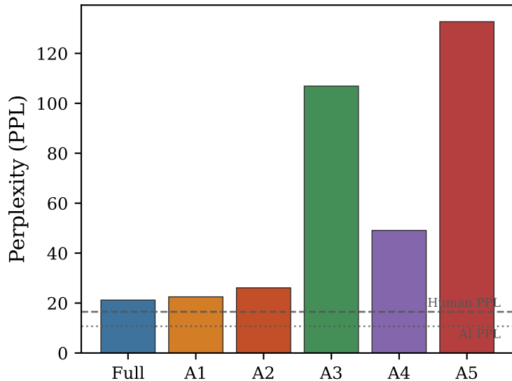
(b) Perplexity ( \gamma=7.0 )
