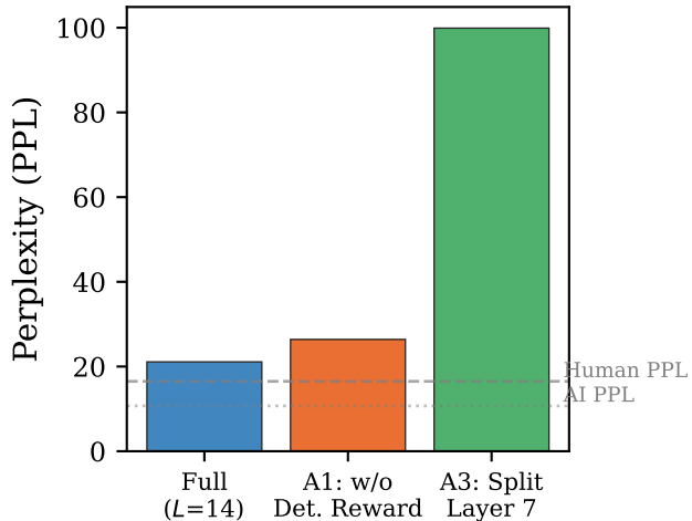
(b) Perplexity ( \gamma=6.5 )
