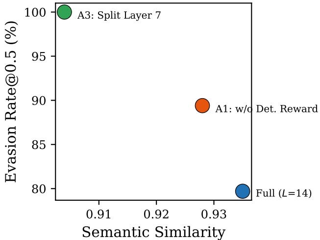
(a) Similarity vs Evasion ( \gamma=6.5 )
