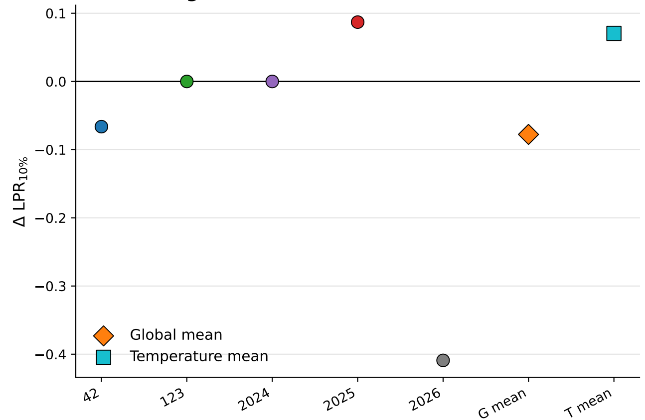
b2 Held-out test batteries (n=4): Near-EOL
