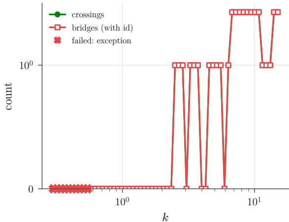
(a) what the recipe finds ( b = 1 saddle)
