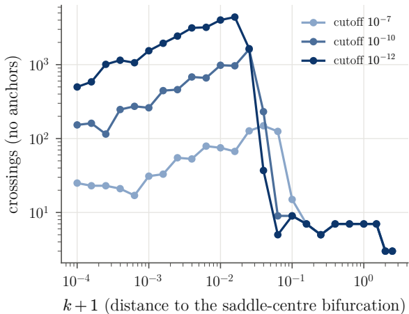
(a) crossings near tangency
