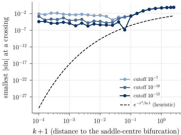
(b) crossing angle vs splitting
