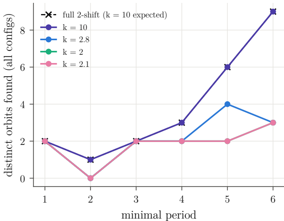
(a) orbits found vs the horseshoe count
