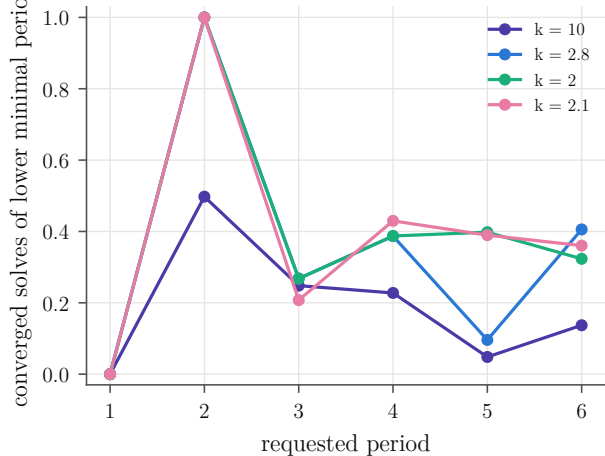
(b) wrong-period rate
