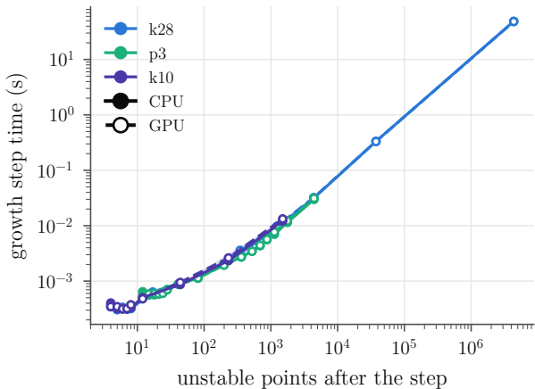
(a) per-step growth (median of 3, IQR band)
