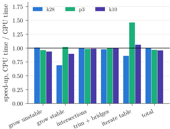
(b) speed-up per stage (median times)
