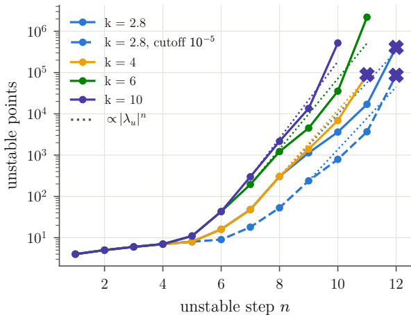
(a) point count
