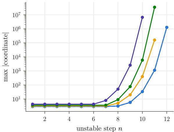
(b) escape to infinity
