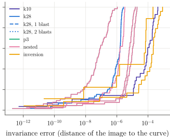
(b) stable manifolds (one line per branch)
