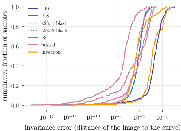
(a) unstable manifolds (one line per branch)
