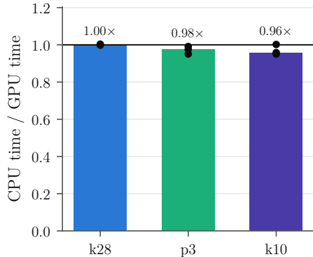
(b) end-to-end GPU speed-up (E2)
