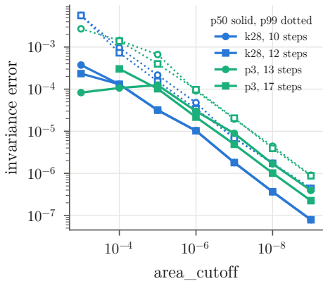
(c) accuracy knob (E4)
