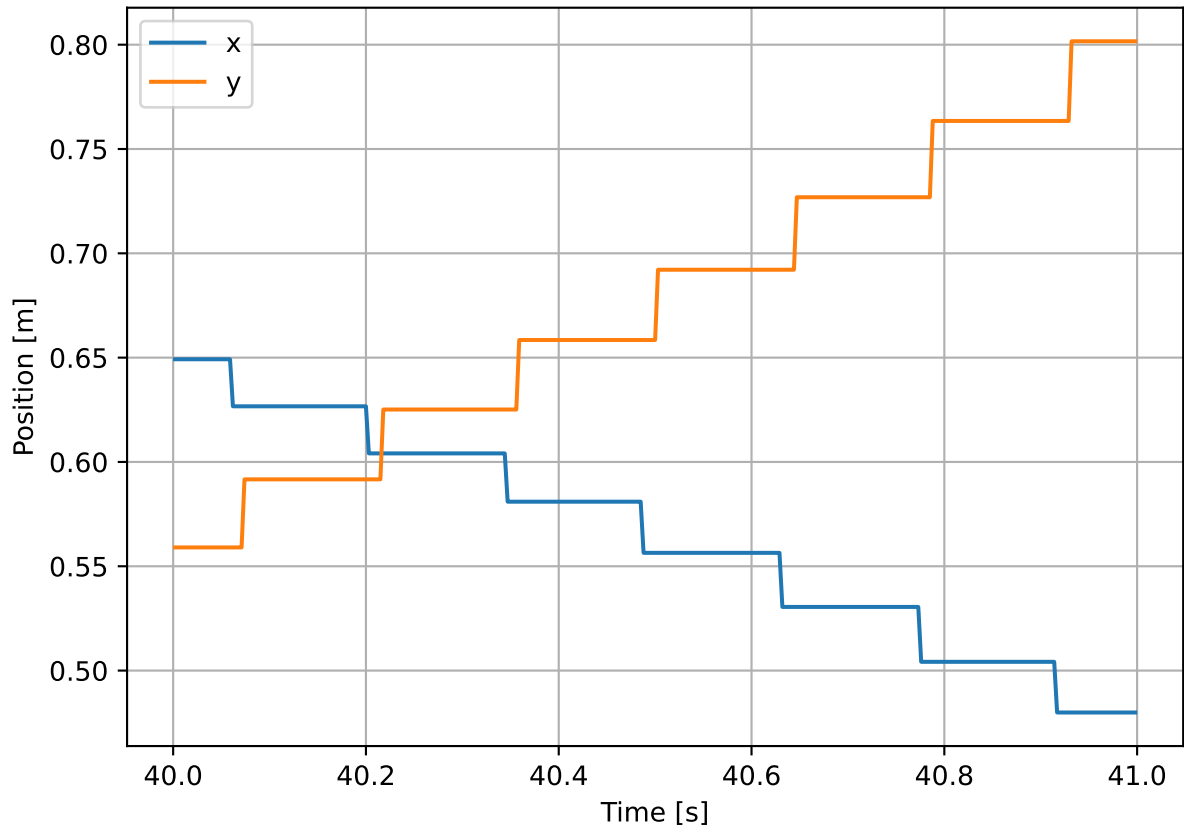
Robot trajectory - 1s window
