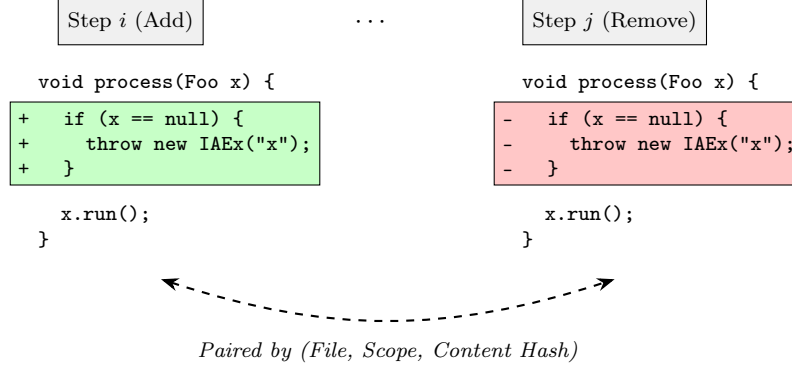
Figure 3.3: Rework detection for an added chunk that is later removed. The detector pairs the two hunks using their ( file, scope, content-hash ) tuple. The synthesiser then builds a shorter alternative trajectory by removing both halves of the rework and preserving the other intermediate edits.
