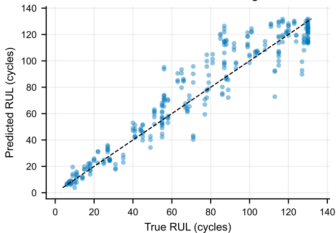
FD003: Gradient Boosting
