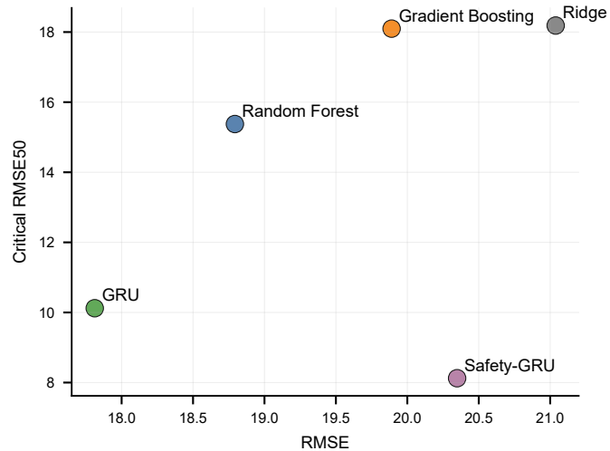
FD004
