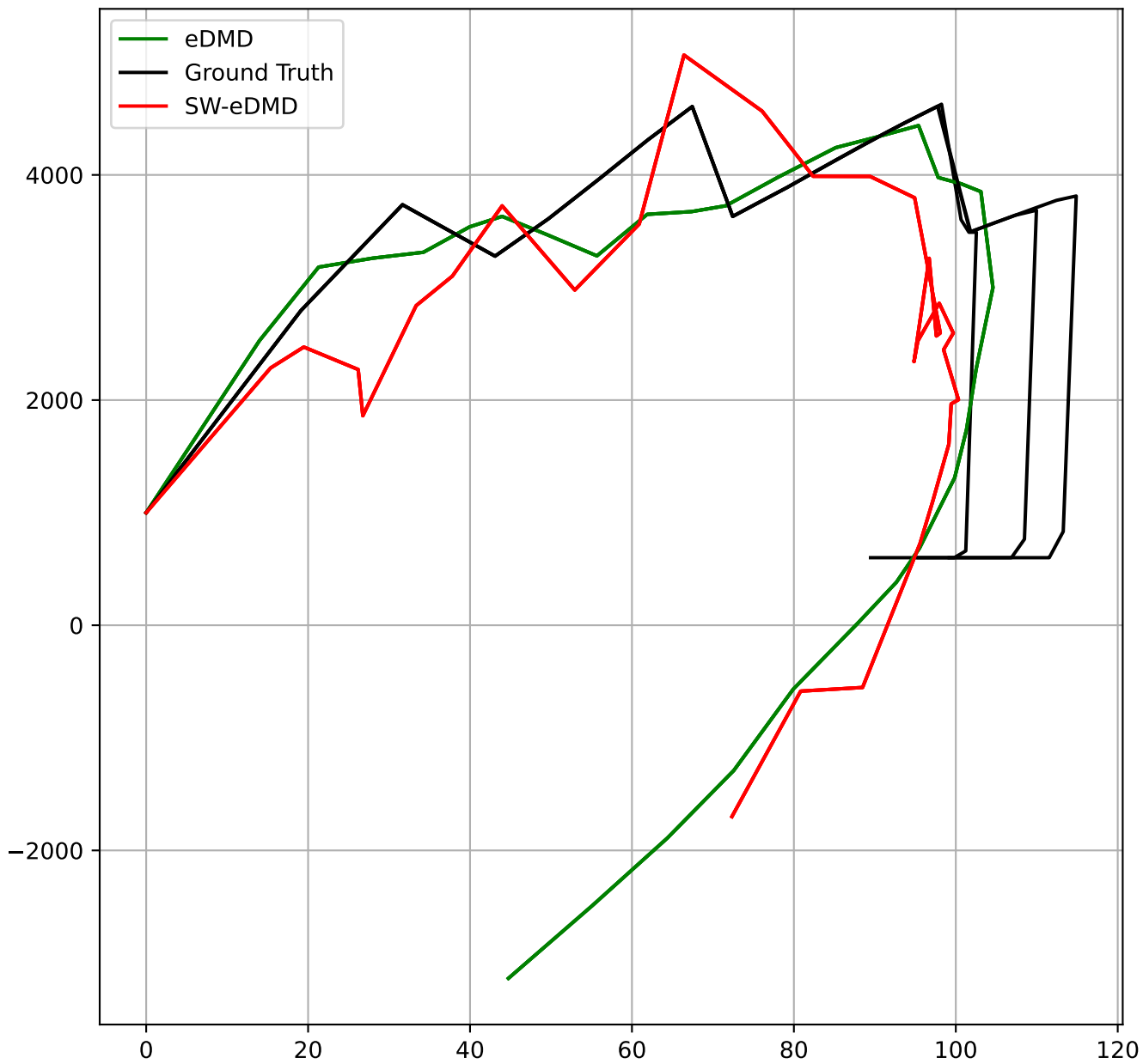
eDMD Results
