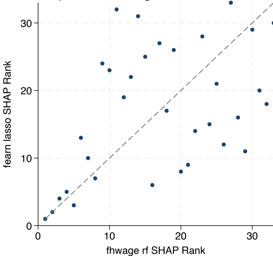
alpha ind: fhwage rf vs fearn lasso
