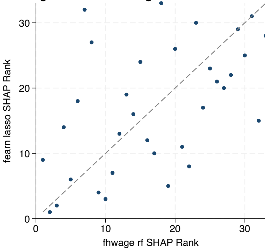
gamma ind: fh wage rf vs fearn lasso
