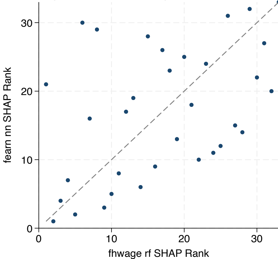
gamma ind: fhwage rf vs fearn nn
