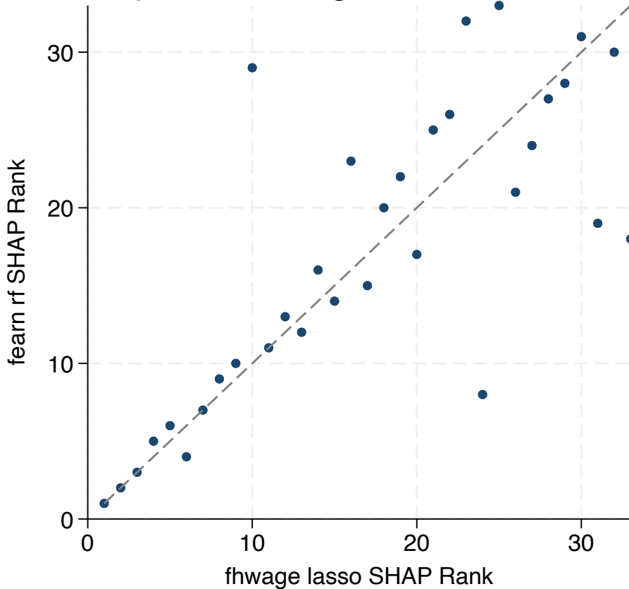
alpha ind: fhwage lasso vs fearn rf
