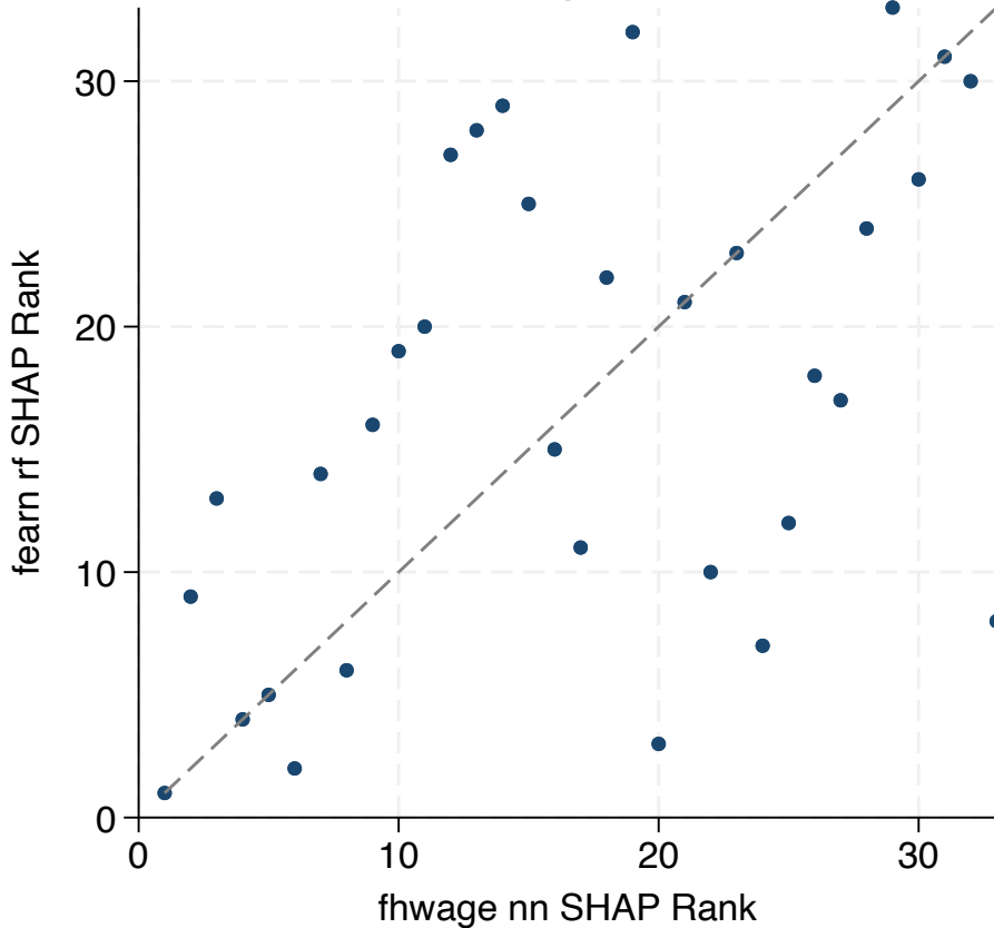
alpha ind: fhwage nn vs fearn rf
