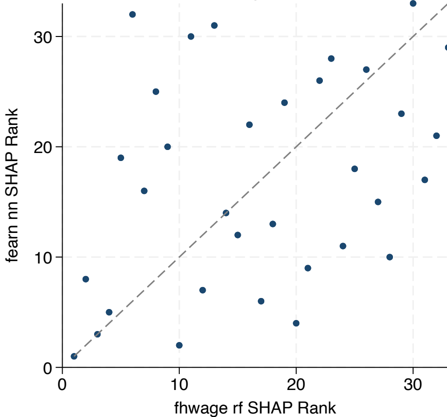
alpha ind: fhwage rf vs fearn nn
