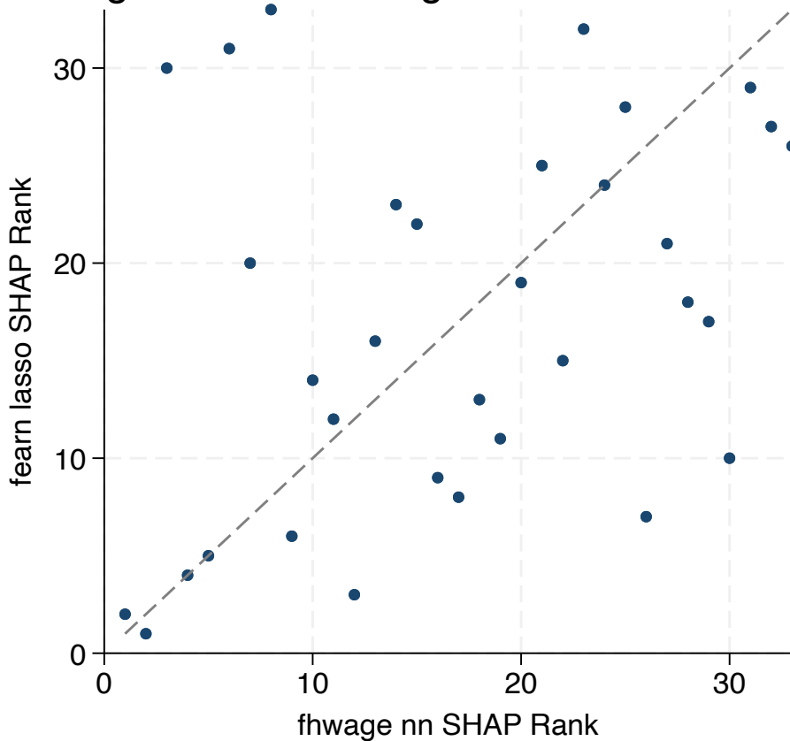
gamma ind: fh wage nn vs fearn lasso
