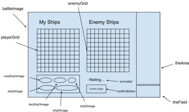
Figure 2: The user drags and drops ships on the “My Ships” grid, then presses Confirm Ships. Players takes turns pressing grid squares on the “Enemy Ships” grid, and are able to send and receive messages through the text field and area
