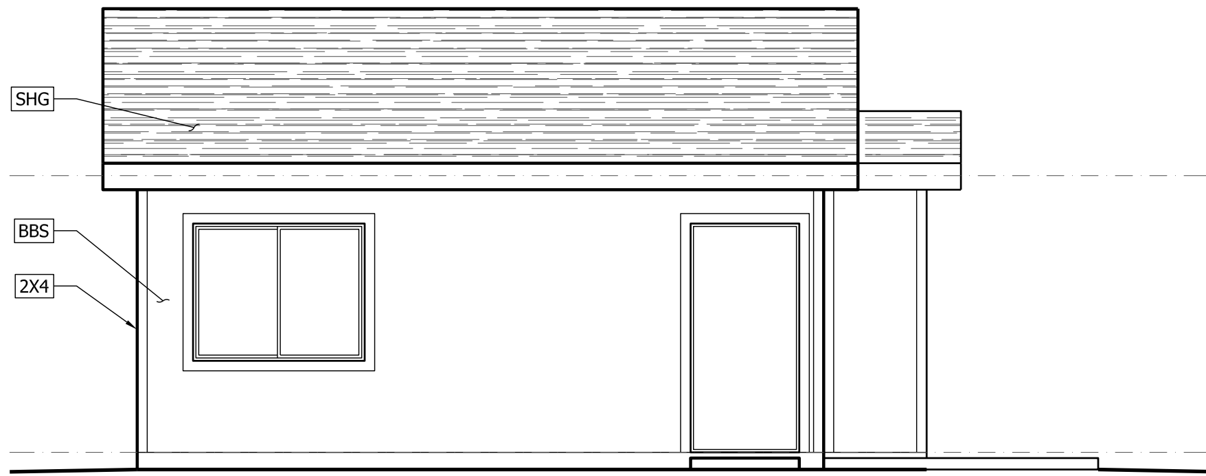
A FRONT ELEVATION
