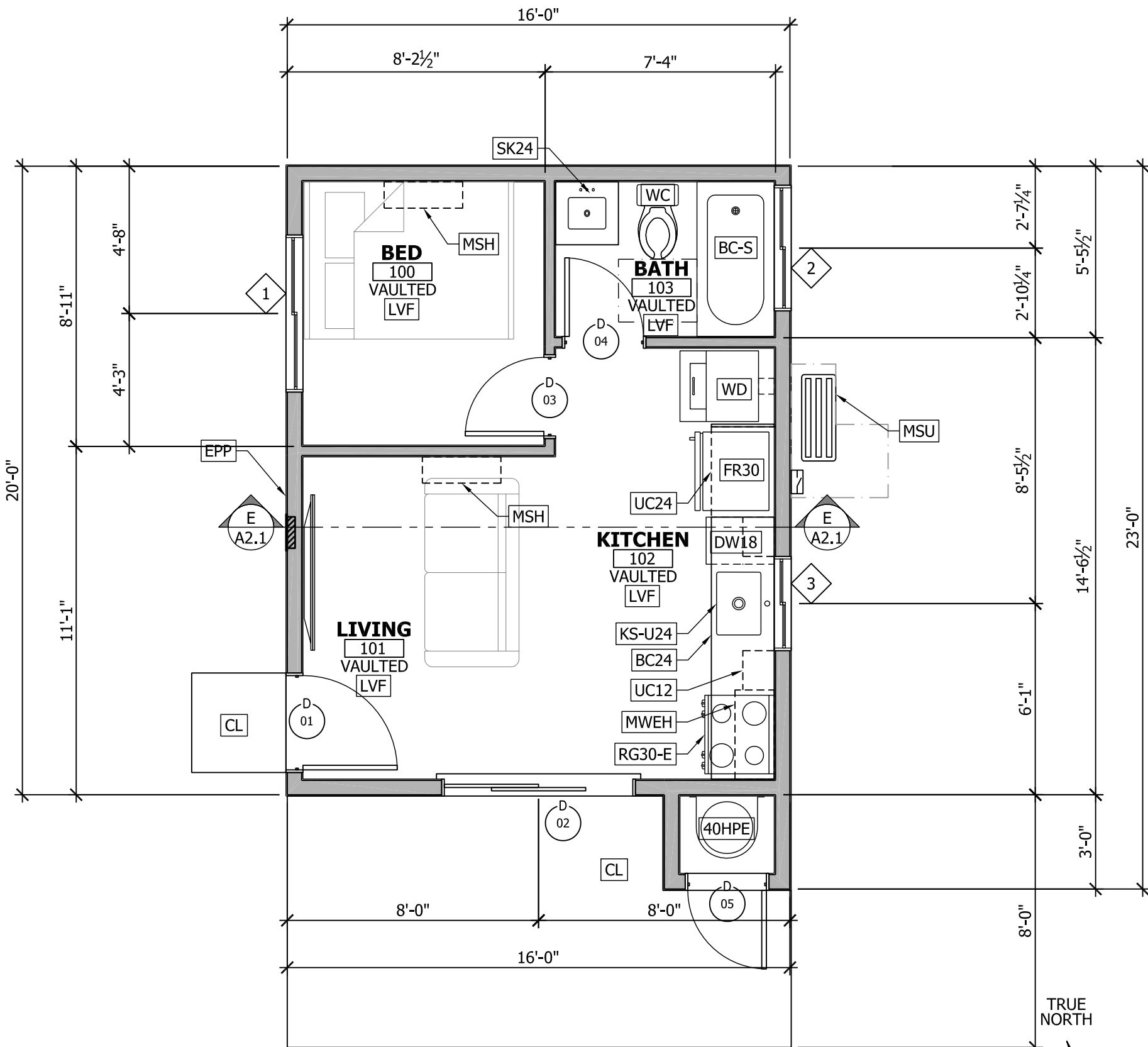
1 FLOOR PLAN #1
