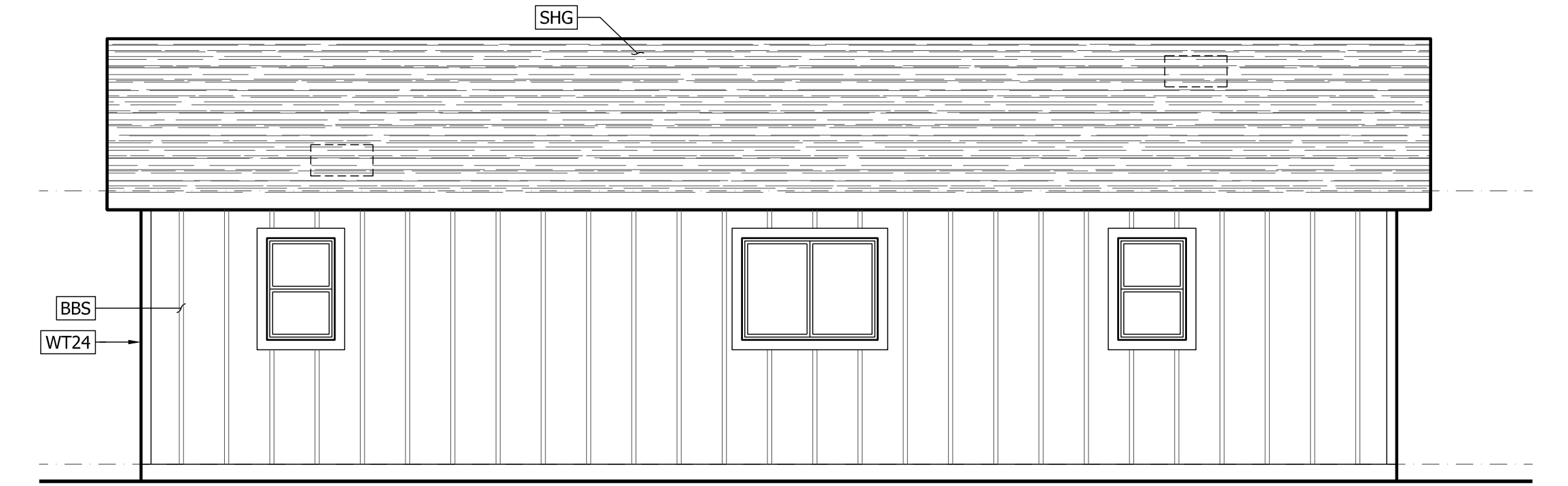
B REAR ELEVATION 1 1/4" = 1'-0"
