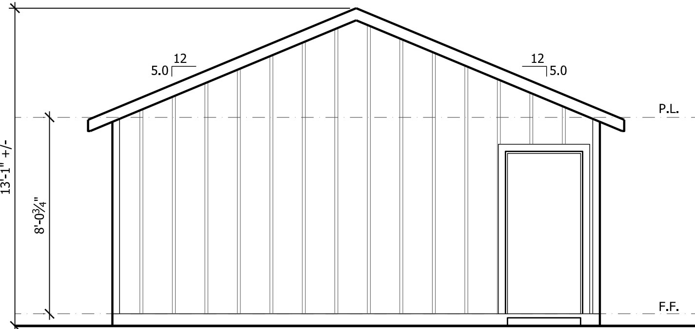
C LEFT ELEVATION 1 1/4" = 1'-0"
