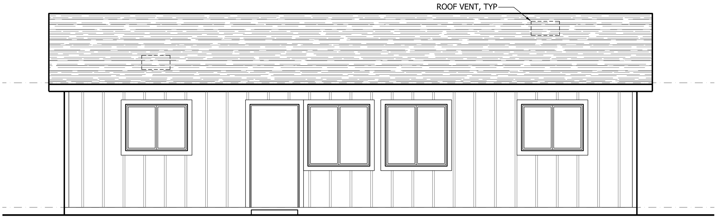
A FRONT ELEVATION 1 1/4" = 1'-0"
