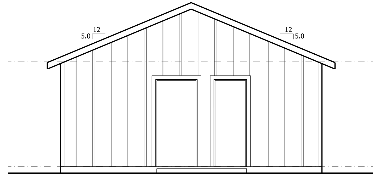
D RIGHT ELEVATION 1 1/4" = 1'-0"
