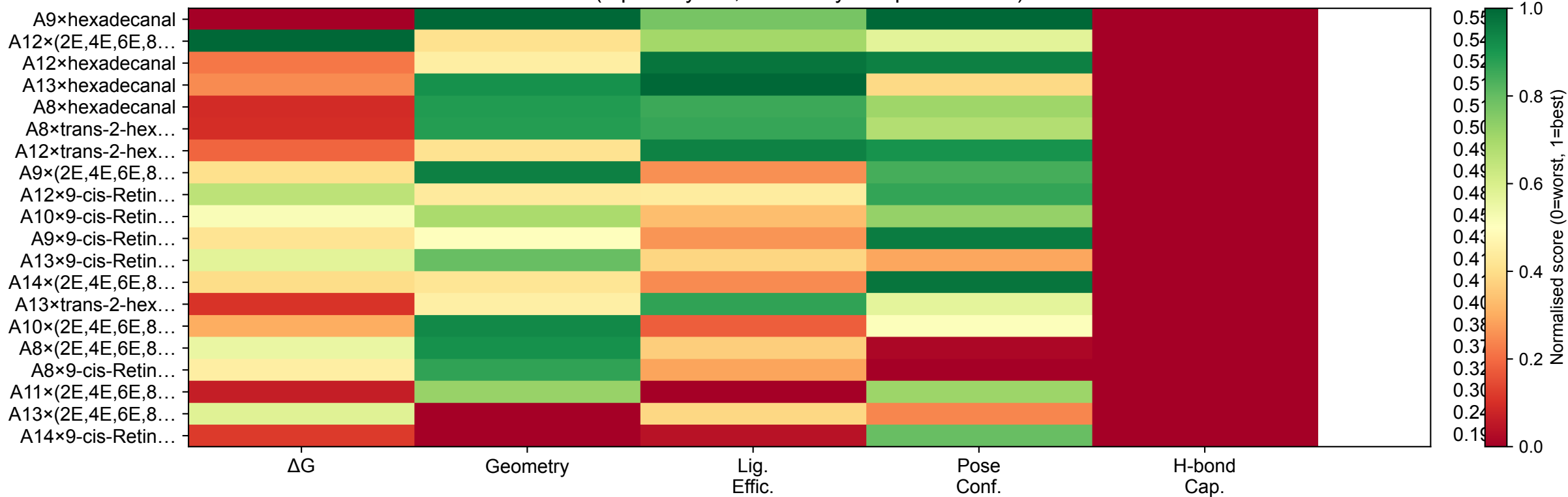
c Multi-criteria decision matrix (top-20 by \Delta G , ranked by composite score)
