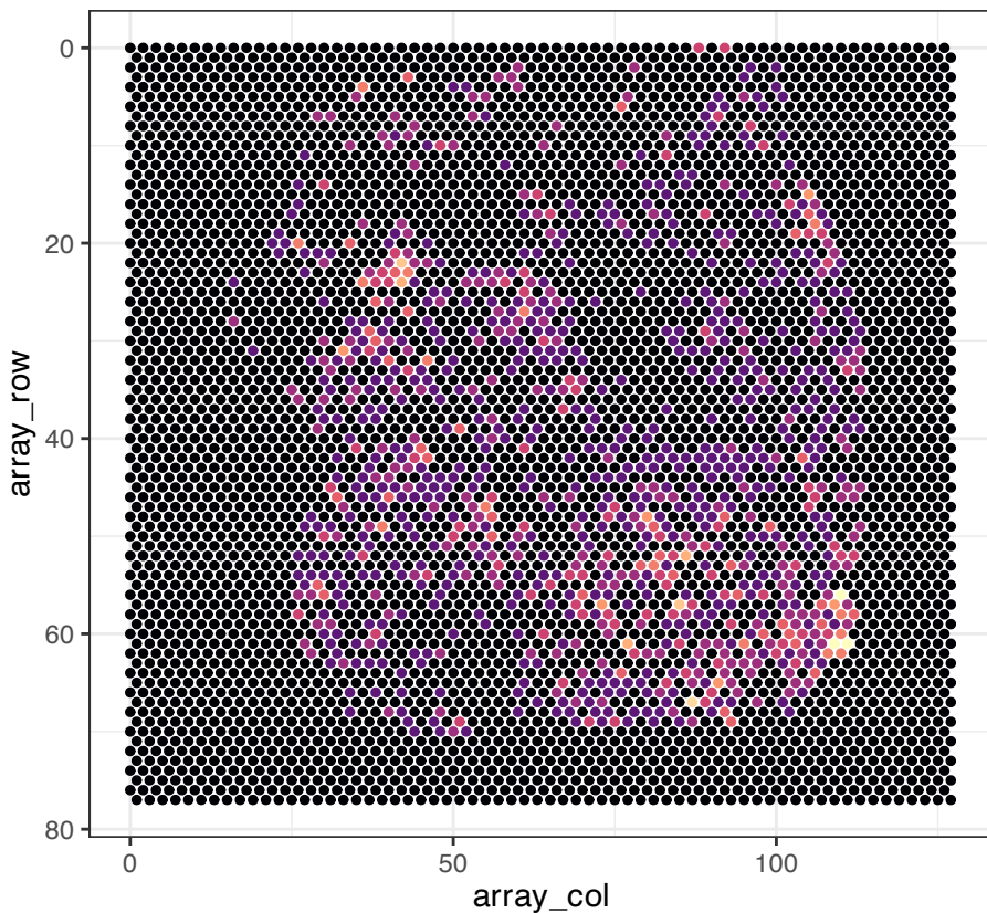
Spatial expression of ENSG00000168542
