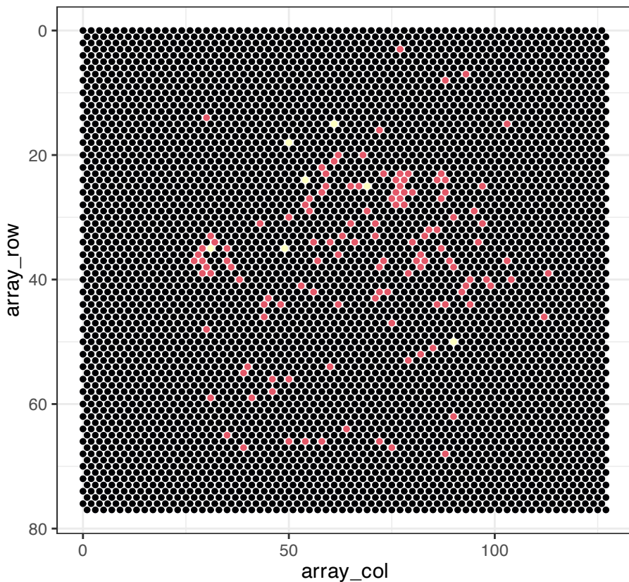
Spatial expression of ENSG00000041982
