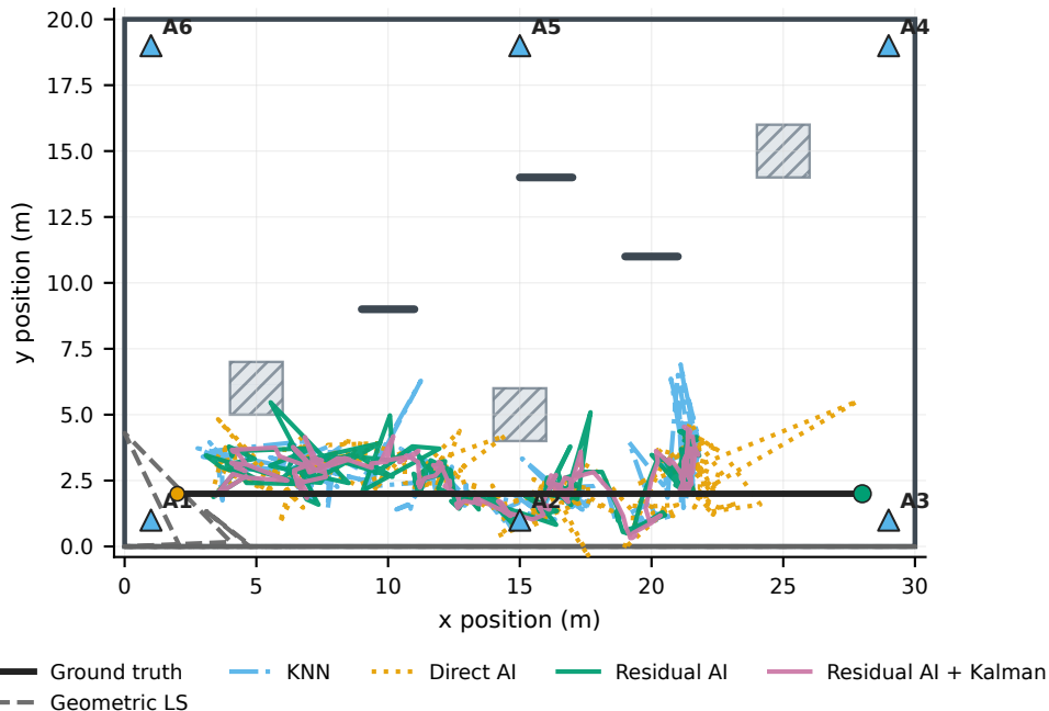
Trajectory localization under the Normal simulation scenario
