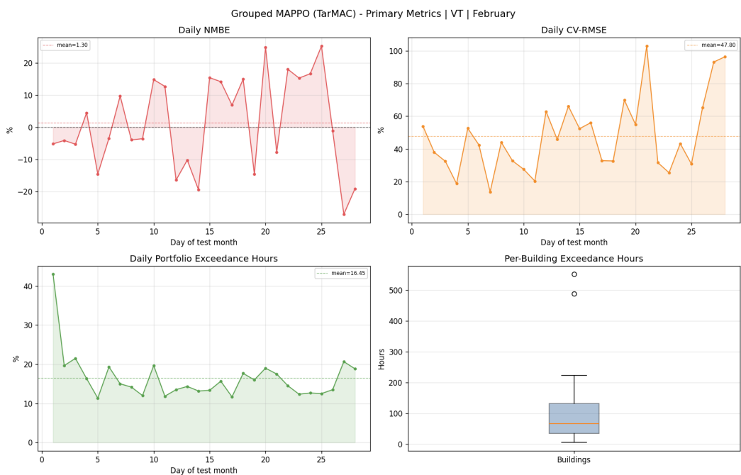
Figure 2: Daily NMBE, CV-RMSE, portfolio comfort exceedance, and the distribution of per-building exceedance hours for the selected Soft Router run. The exported figure retains the TarMAC backbone label.
