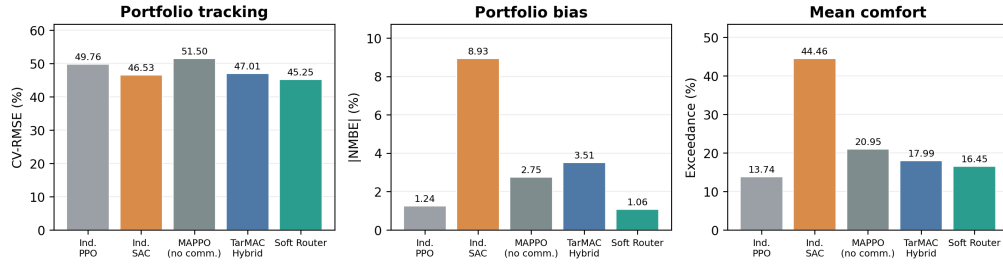
Figure 1: Focused comparison requested from the recorded Vermont runs. The Soft Router bar is the selected seed-0 run built from the seed-42 TarMAC Hybrid experts. PPO has a smaller training budget than the other baselines. Lower is better in all three panels.
