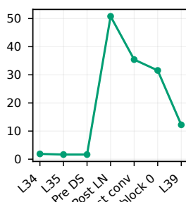
PCA-128 effective rank
