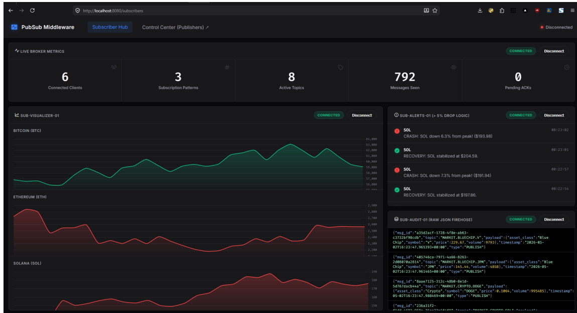
Figure 3: Subscriber Hub Web Interface
