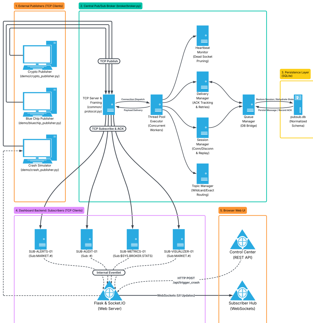
Figure 1: End-to-End System Architecture
