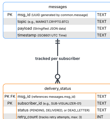
Figure 4: Entity-Relationship (ER) Diagram of the Persistence Layer
