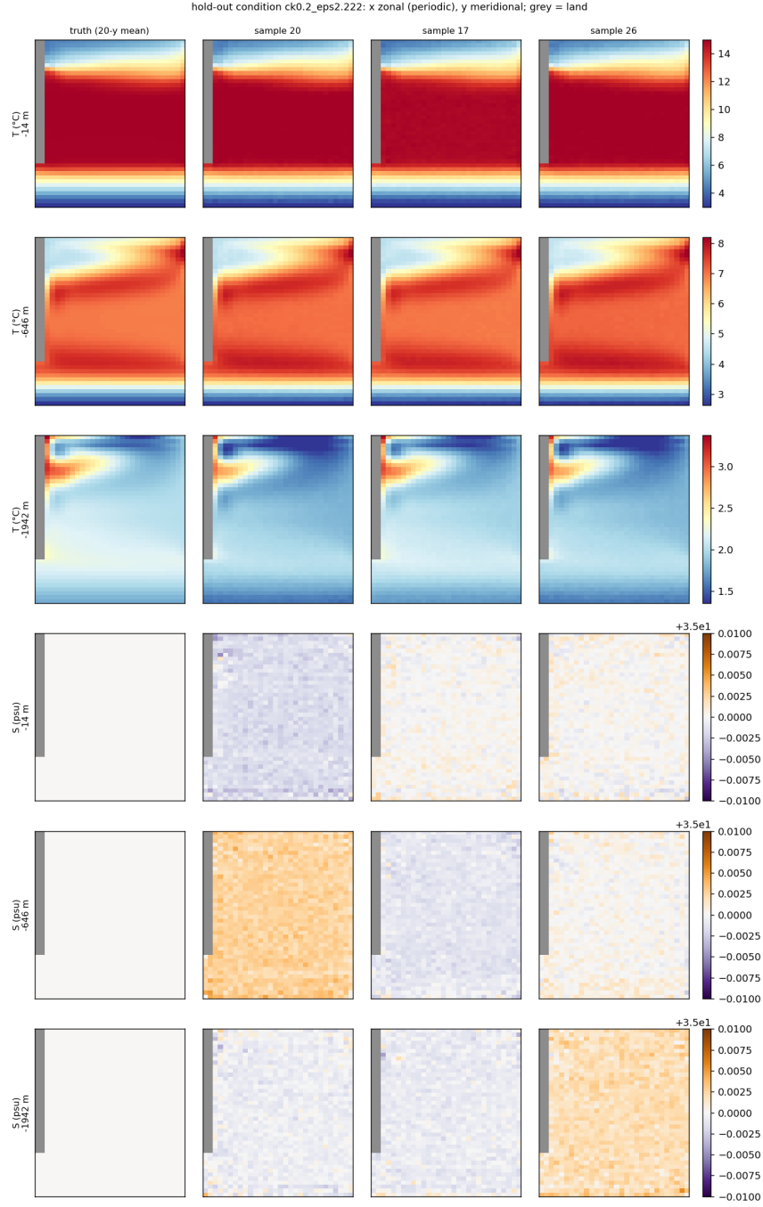
Figure 10: Centre-block split, same condition ( c_k = 0.2 , c_\epsilon = 2.222 , inside the held-out block).
