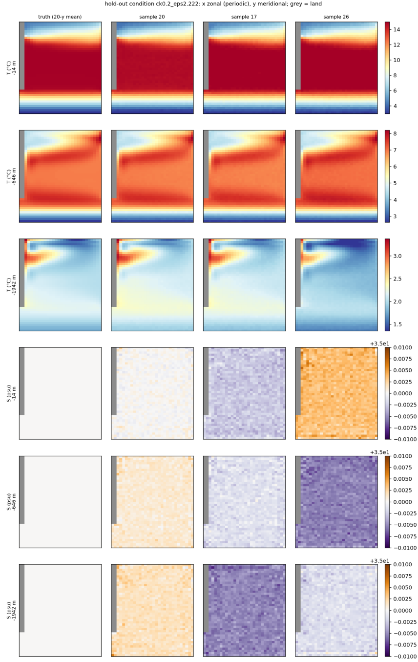
Figure 9: Band-of-three split, same condition ( c_k = 0.2 , c_\epsilon = 2.222 , now in the middle held-out row).
