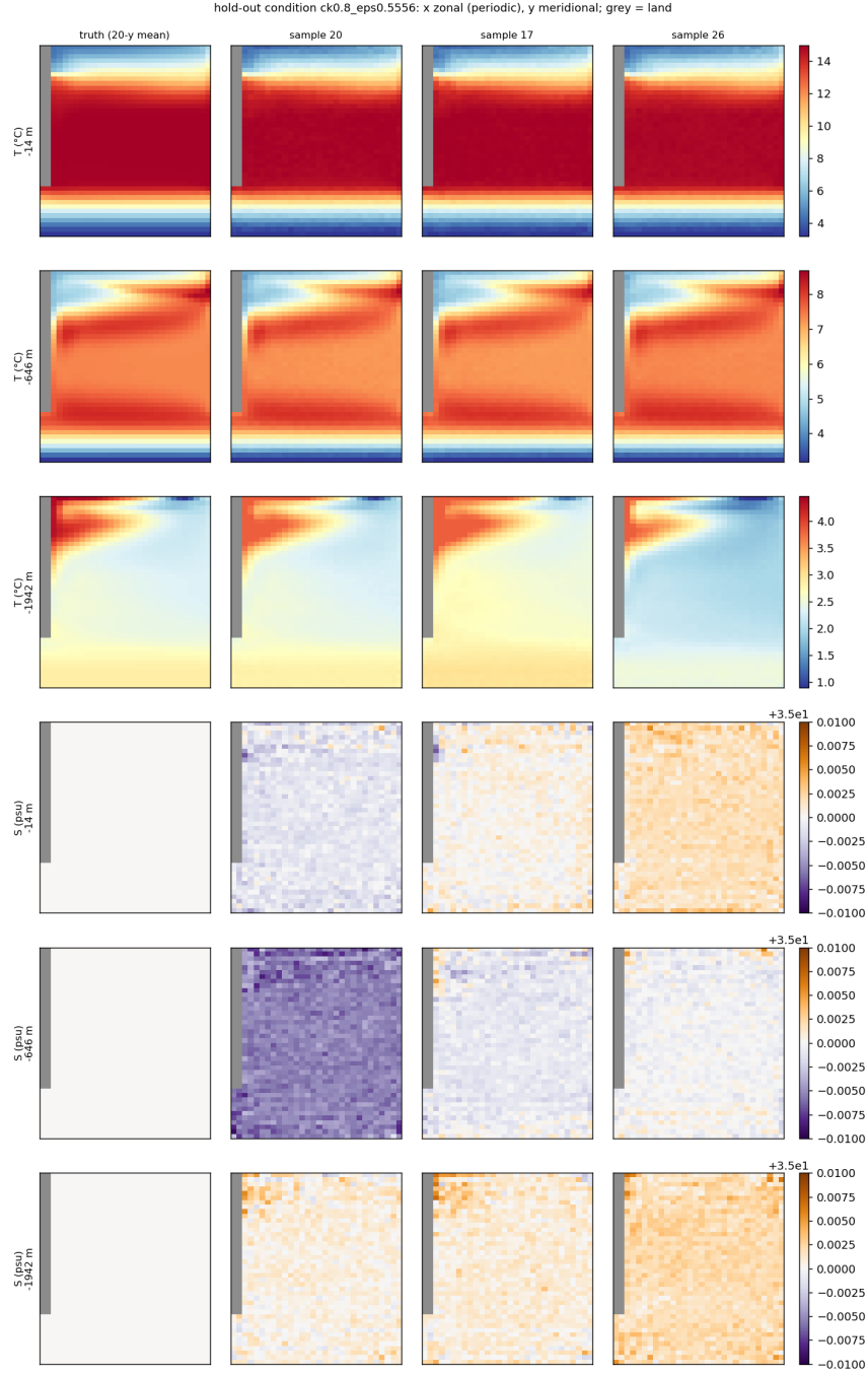
Figure 11: Outer-ring split, c_k = 0.8 , c_\epsilon = 0.5556 (same condition as the top-row split; here the whole outer ring is unseen).
