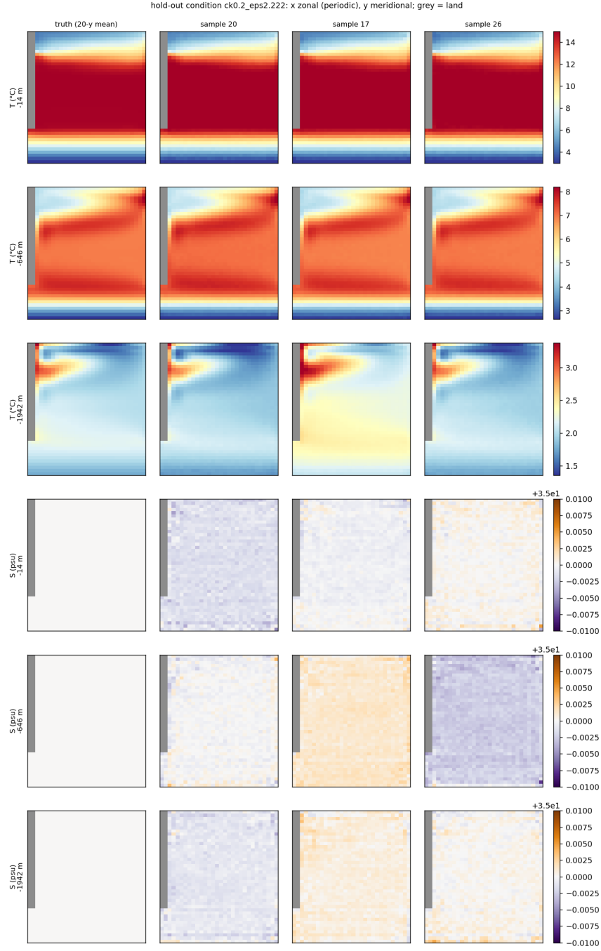
Figure 23: Four-run split, same condition ( c_k = 0.2 , c_\epsilon = 2.222 ).
