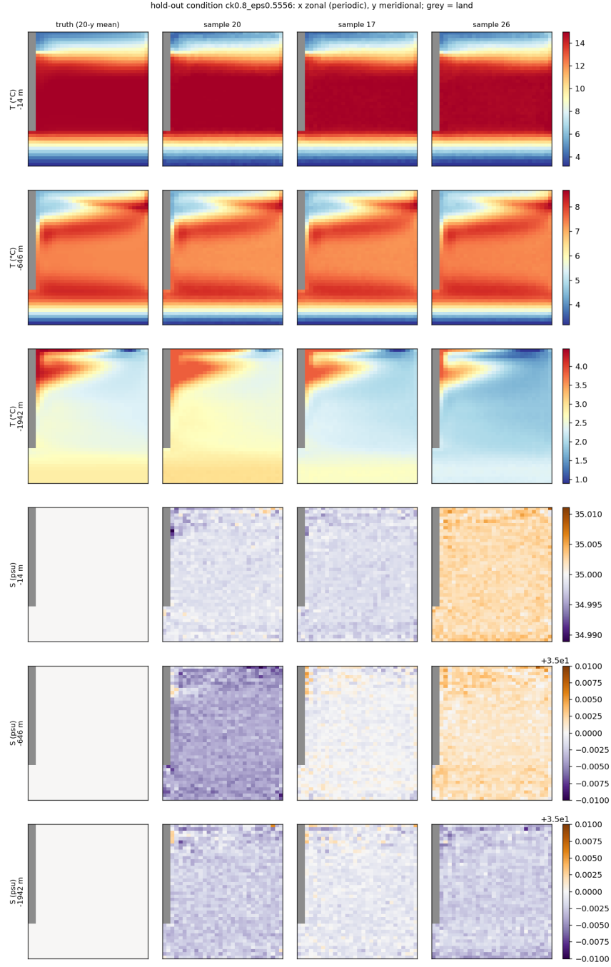
Figure 22: Top-row split, c_k = 0.8 , c_\epsilon = 0.5556 (extrapolation one row above the training grid).
