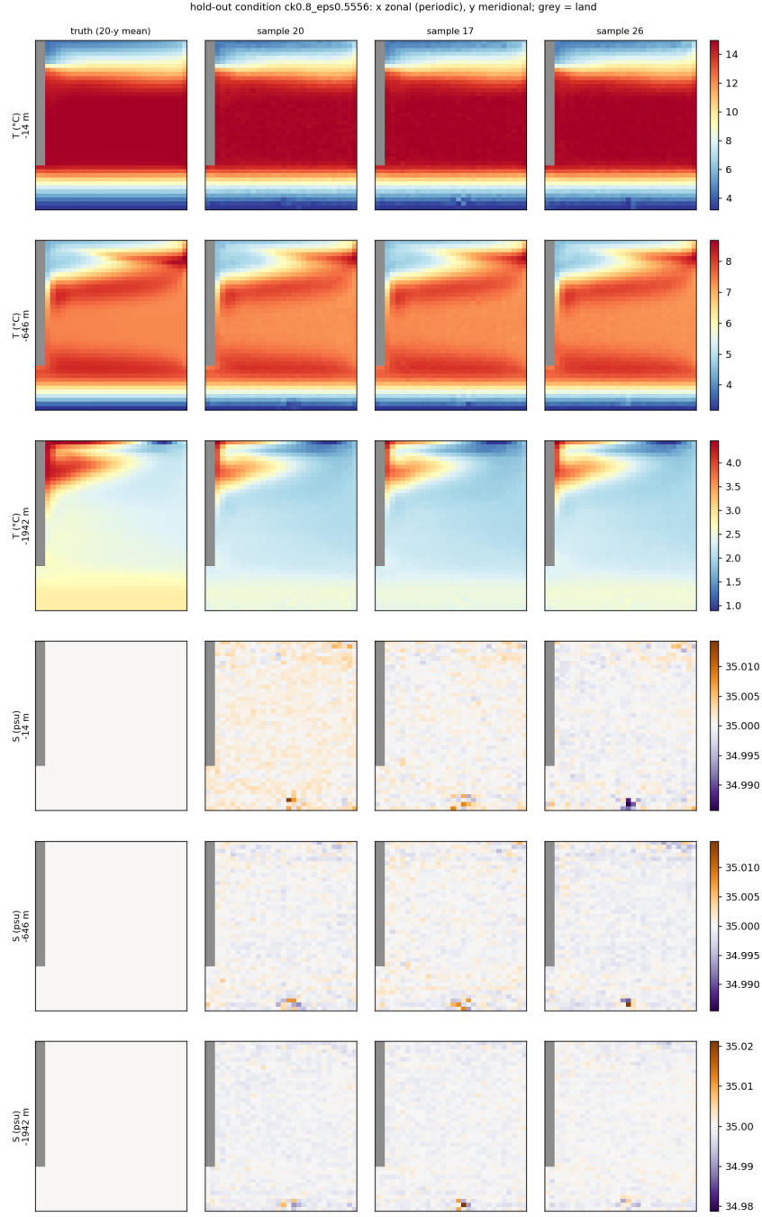
Figure 20: Outer-75 split, v -prediction, no clip, same condition as Figure 19.
