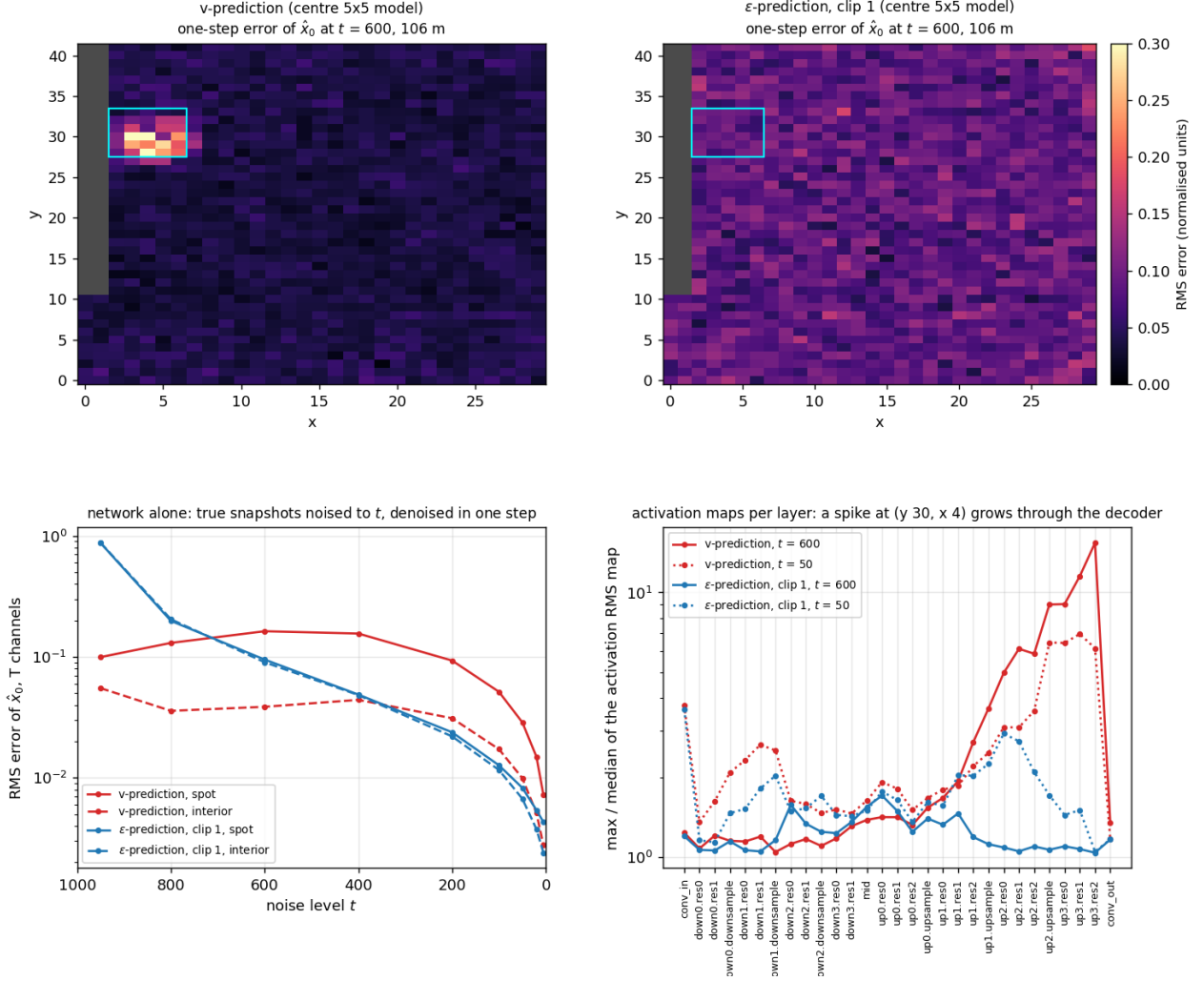
Figure 21: The defect of the centre- 5 \times 5 v model. Top: RMS error of the one-step clean-state estimate for eight true snapshots of a held-out run noised to t = 600 , at 106 m, for the v network (left) and the \epsilon network (right); cyan box: the patch. Bottom left: the same error in the patch and in an interior box as a function of t . Bottom right: maximum over median of each layer's activation map (RMS over channels, mean over the eight inputs) at t = 600 and 50: the spike appears in the second decoder block and grows through the decoder; the \epsilon network stays flat.
