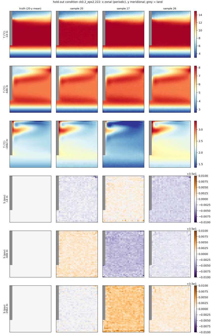
Figure 13: Centre- 5 \times 5 split, same condition ( c_k = 0.2 , c_\epsilon = 2.222 , inside the held-out block).
