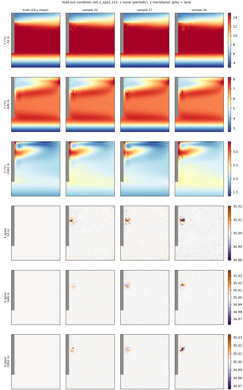
Figure 17: Centre- 5 \times 5 split, v -prediction, no clip, same condition as Figure 16: the samples are far less noisy.
