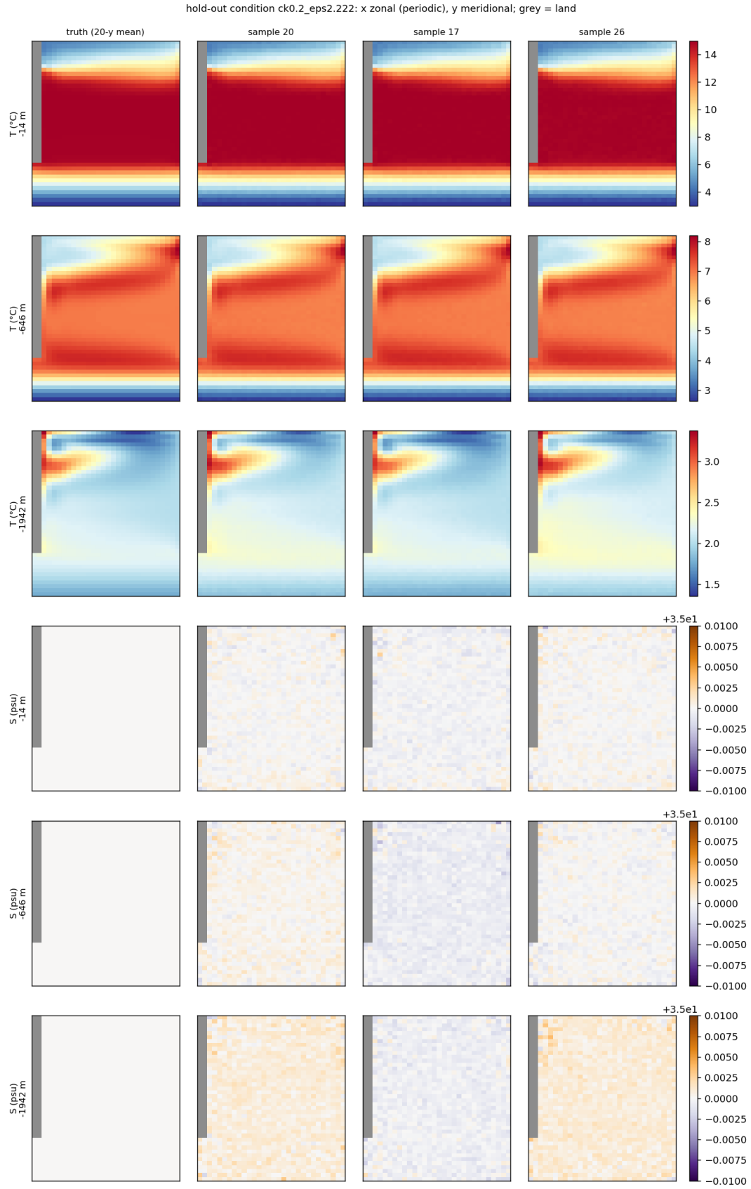
Figure 18: Centre 5 \times 5 , v -prediction with the loss on the water cells, same condition and samples as Figure 17: the patch is gone and S stays within 0.01 psu.
