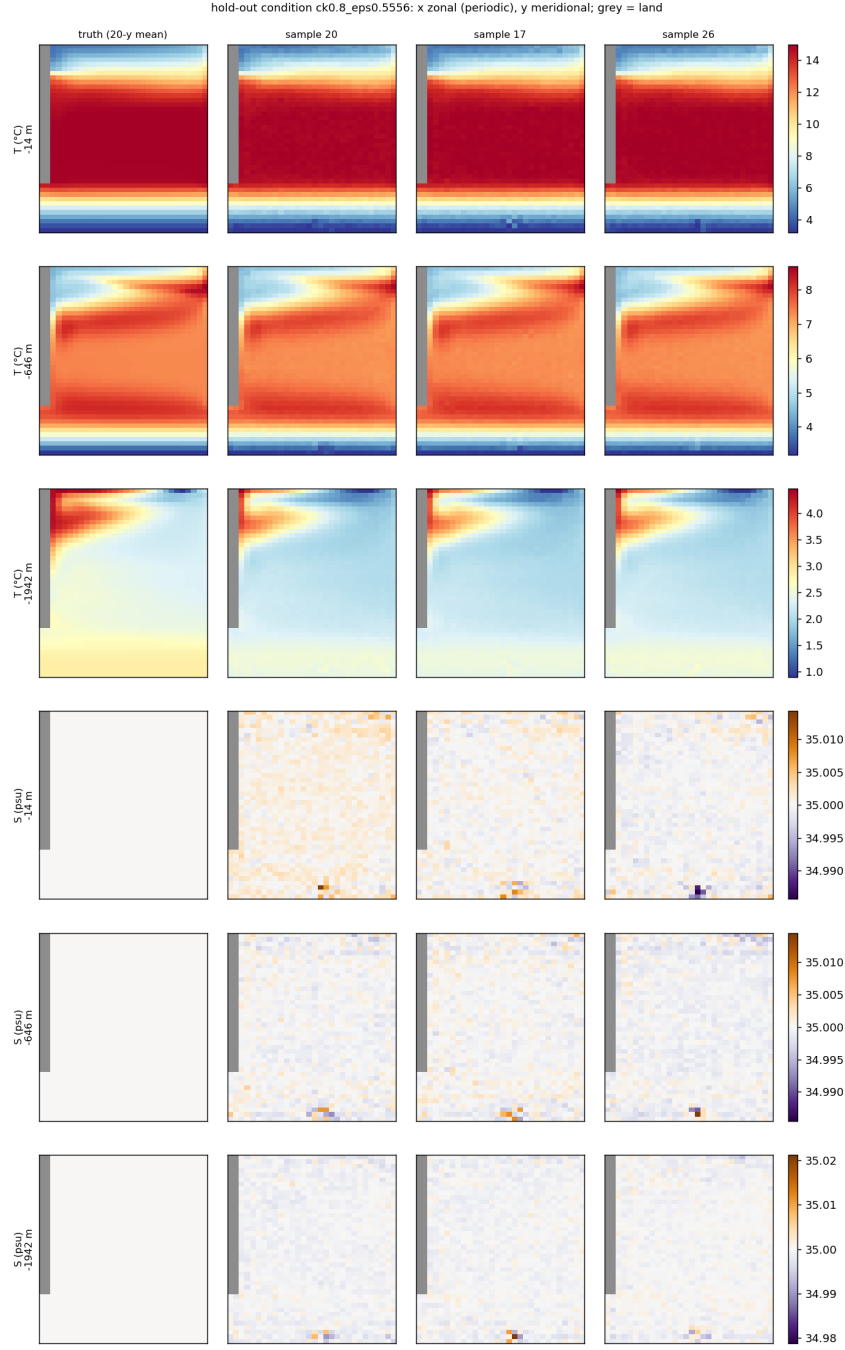
Figure 22: Outer-75 split, v -prediction, no clip, same condition as Figure 21.
