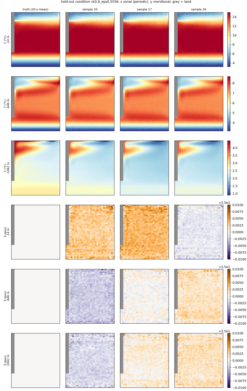
Figure 21: Outer-75 split, c_k = 0.8 , c_\epsilon = 0.5556 (training on the 5 \times 5 centre only).
