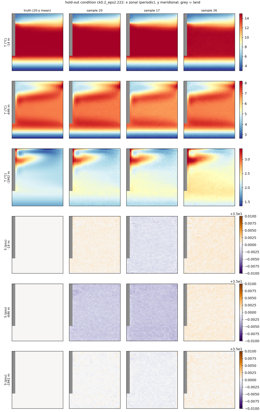
Figure 9: Same condition as Figure 8, min-max normalisation , same sampler.
