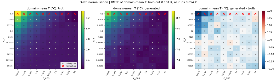
(a) Domain-mean T over the grid.
