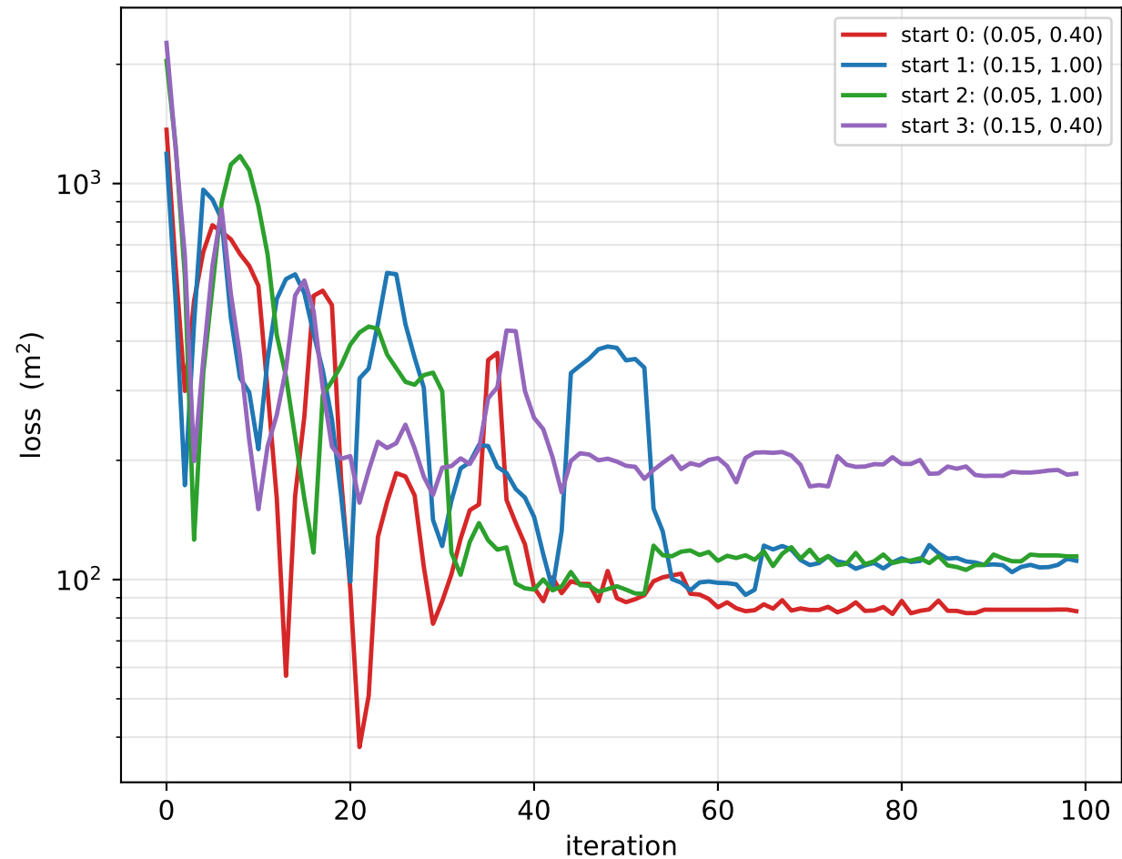
Loss during optimization
