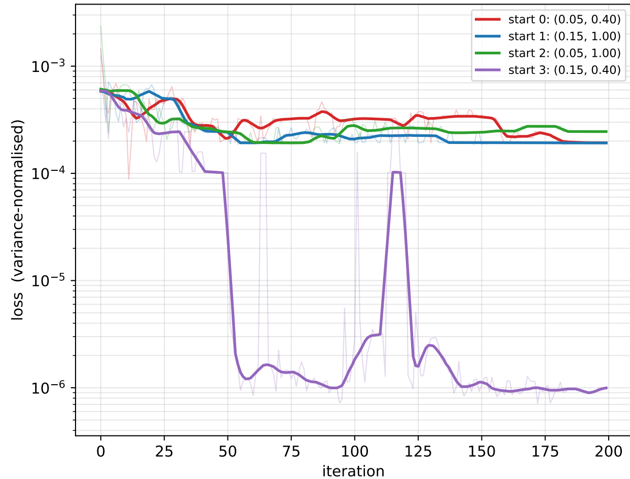
Loss during optimization (bold: rolling median over 9 iterations)
