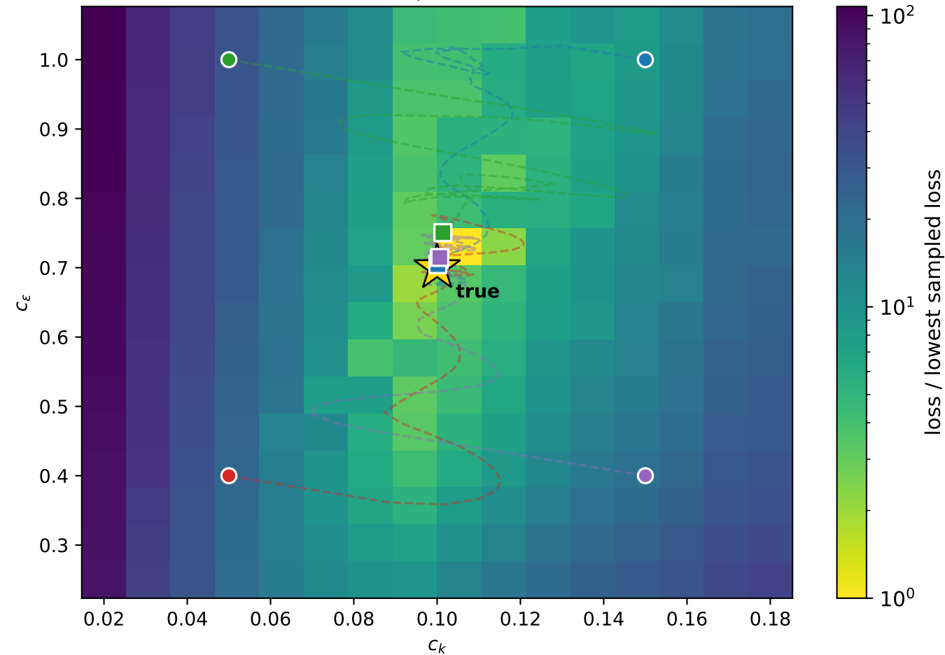
Loss landscape and gradient descent paths (circles: starts, squares: final iterates)
