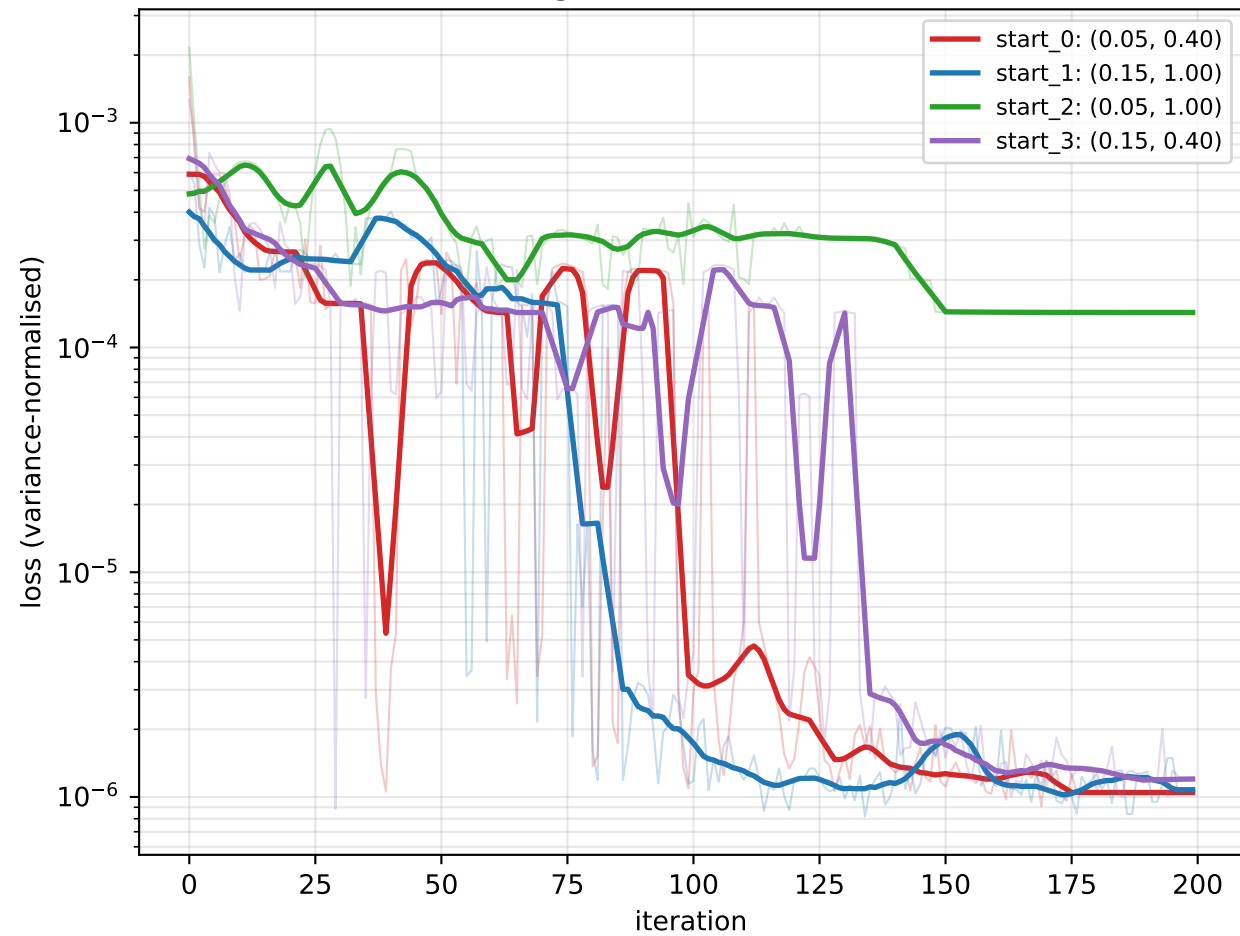
Loss during optimization (bold: rolling median over 9 iterations)
