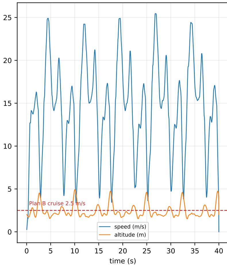
one 40 s episode: 59 gates, laps 7.35-7.47 s, no crash
