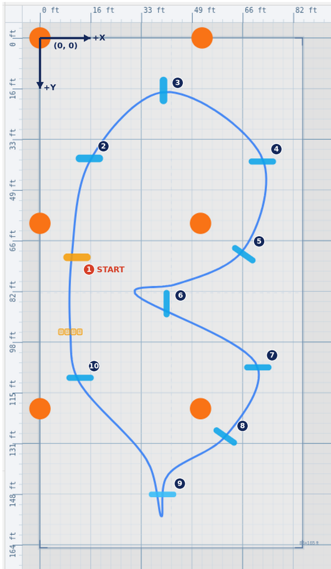
Bird's-eye view of the track. The blue line is the racing line; numbered markers identify each gate. Grid squares are 16.4 ft.
