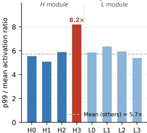
A LIF threshold diagnostic
