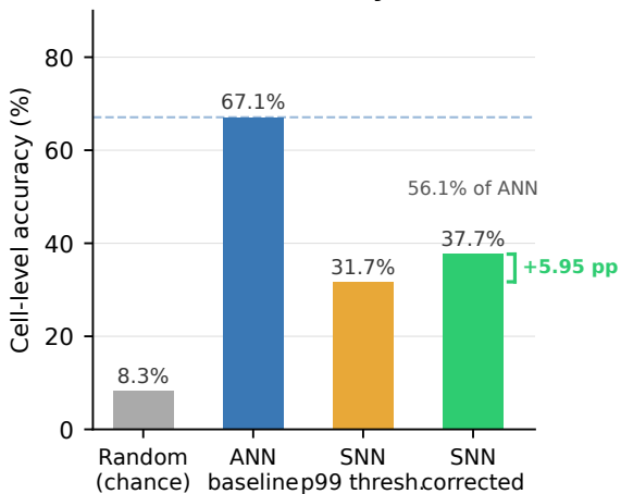
B Cell-level accuracy
