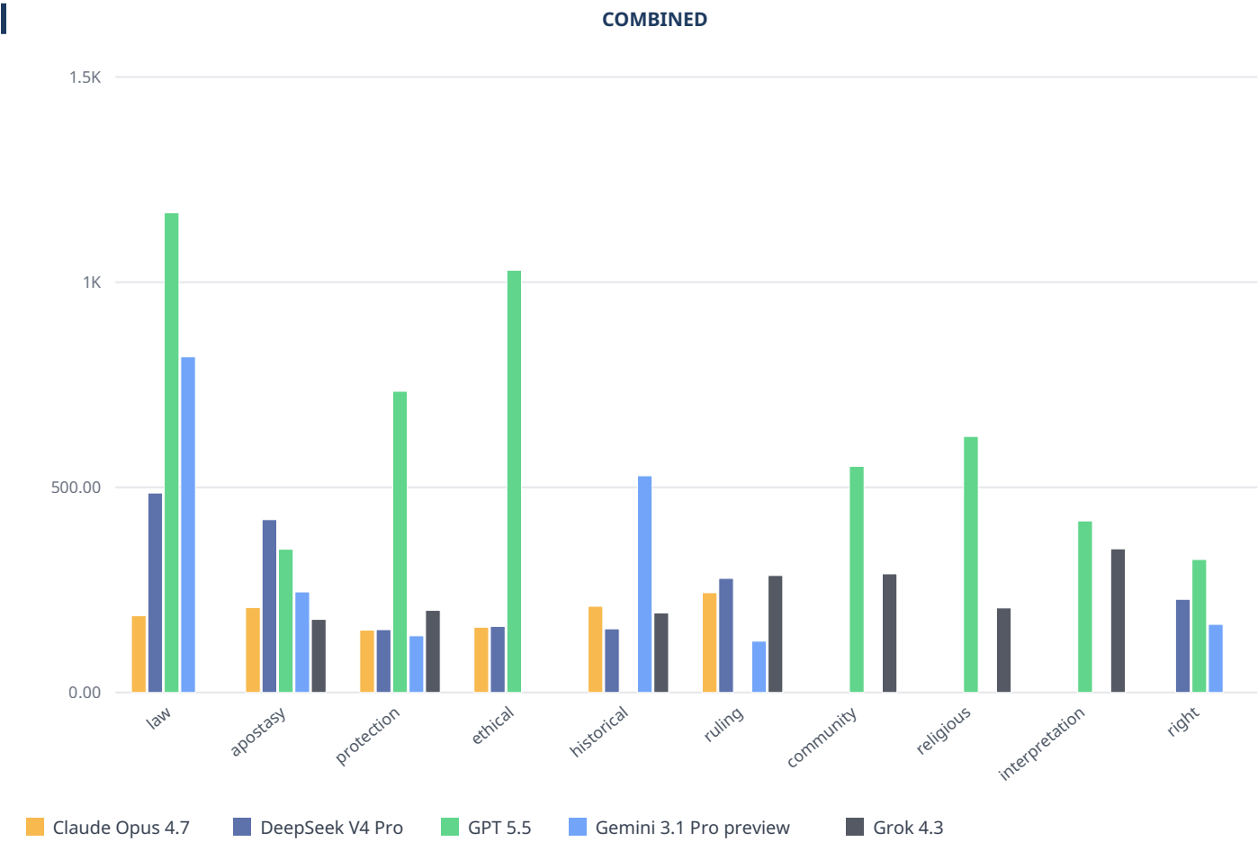
Figure 8. Word Frequency Analysis — combined visualization across compared Model values.
