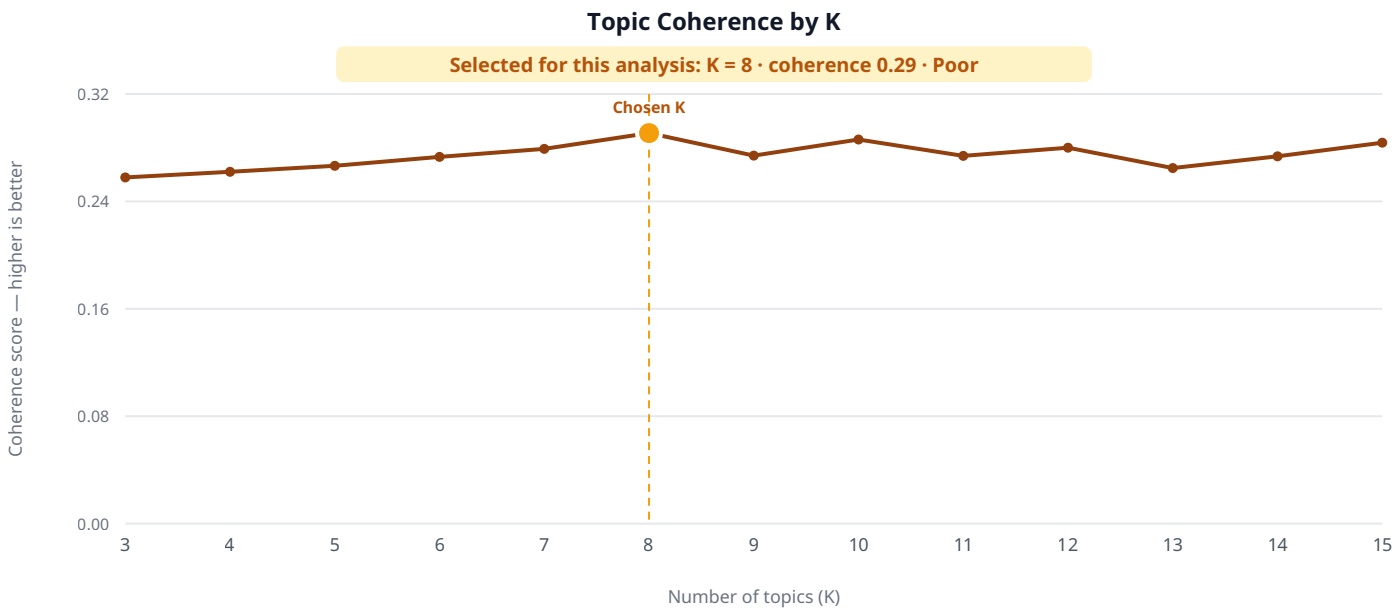
Figure 7. Topic coherence (c_v) across candidate topic counts K from the K search.
