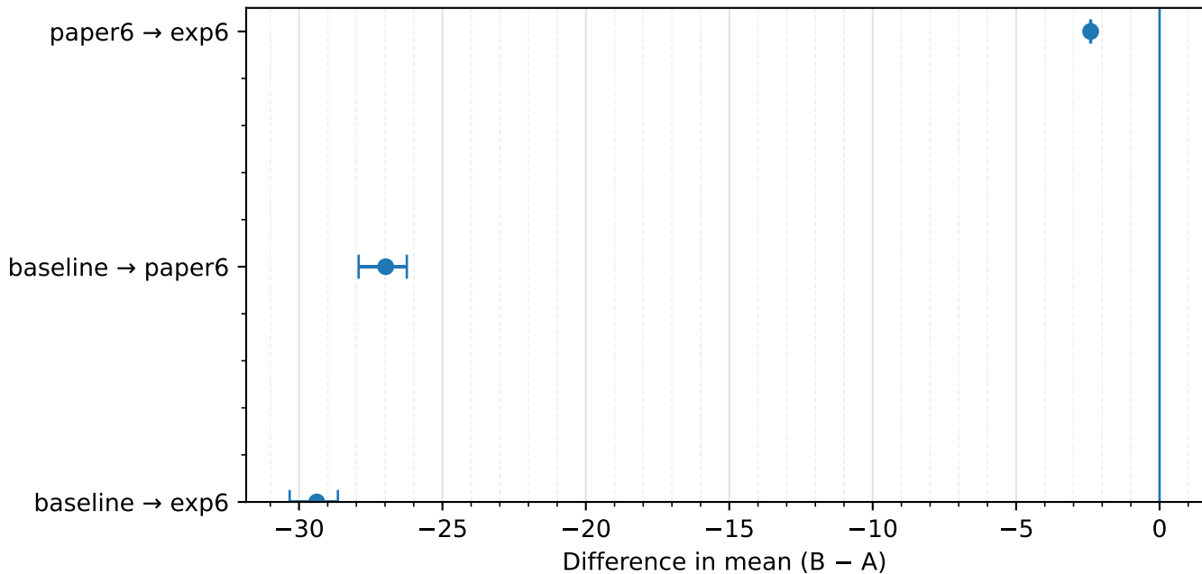
Tracking MAE (deg): pairwise differences (95% bootstrap CI)
