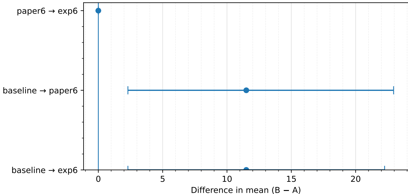
Episode length (steps): pairwise differences (95% bootstrap CI)
