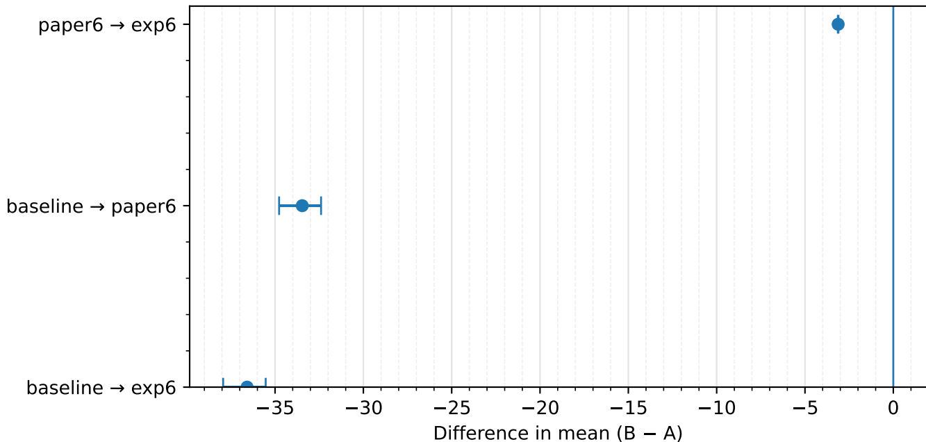
Tracking RMSE (deg): pairwise differences (95% bootstrap CI)
