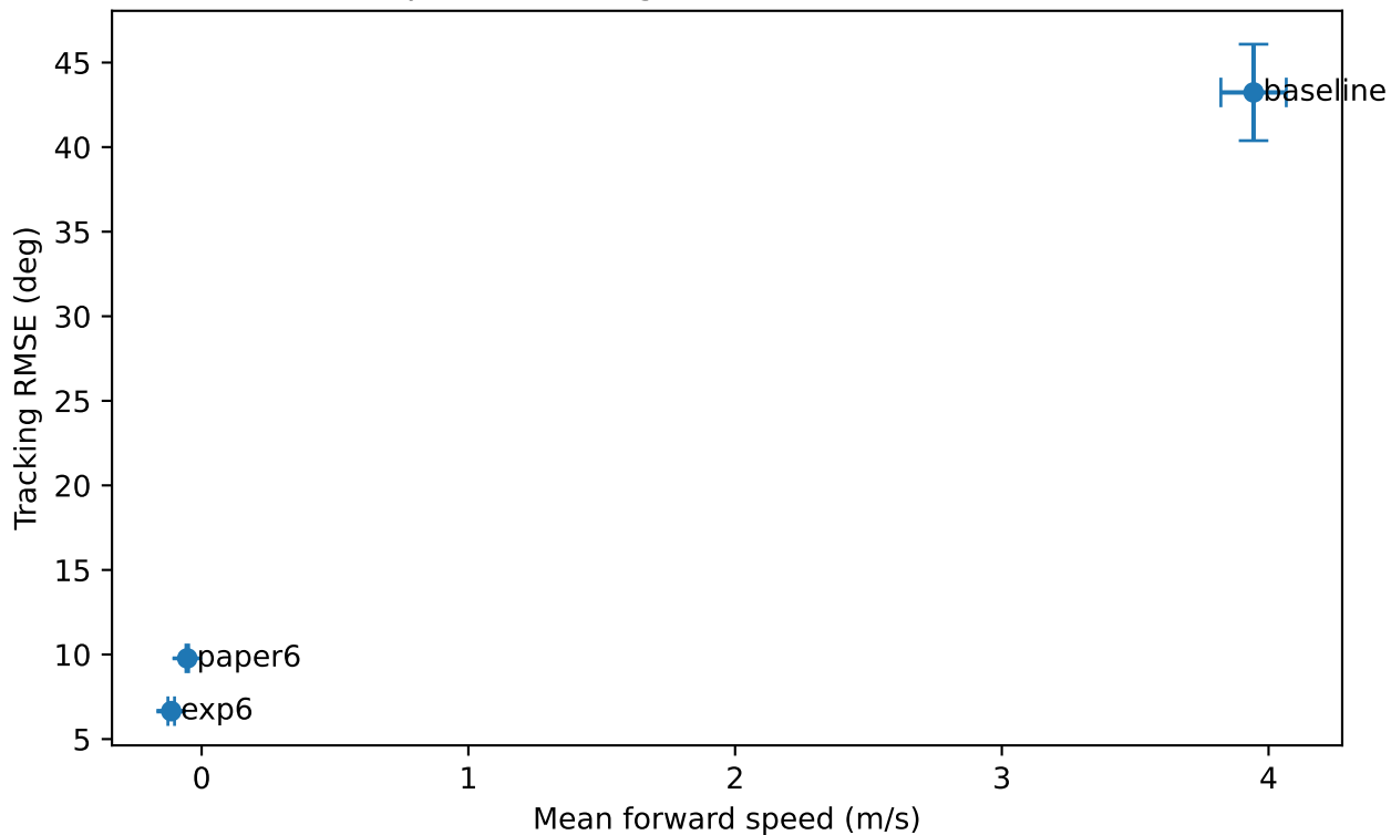
Speed-tracking trade-off (mean \pm std)
