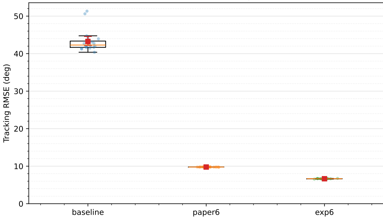
Tracking RMSE (deg) (per-episode) Mean \pm 95% bootstrap CI
