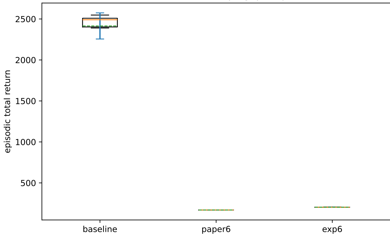
Total return (env + shaping, per-episode)
