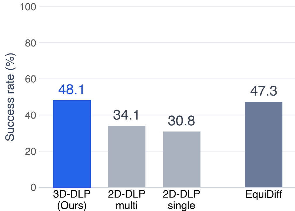
MimicGen
