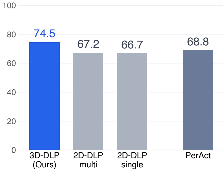
RLBench
