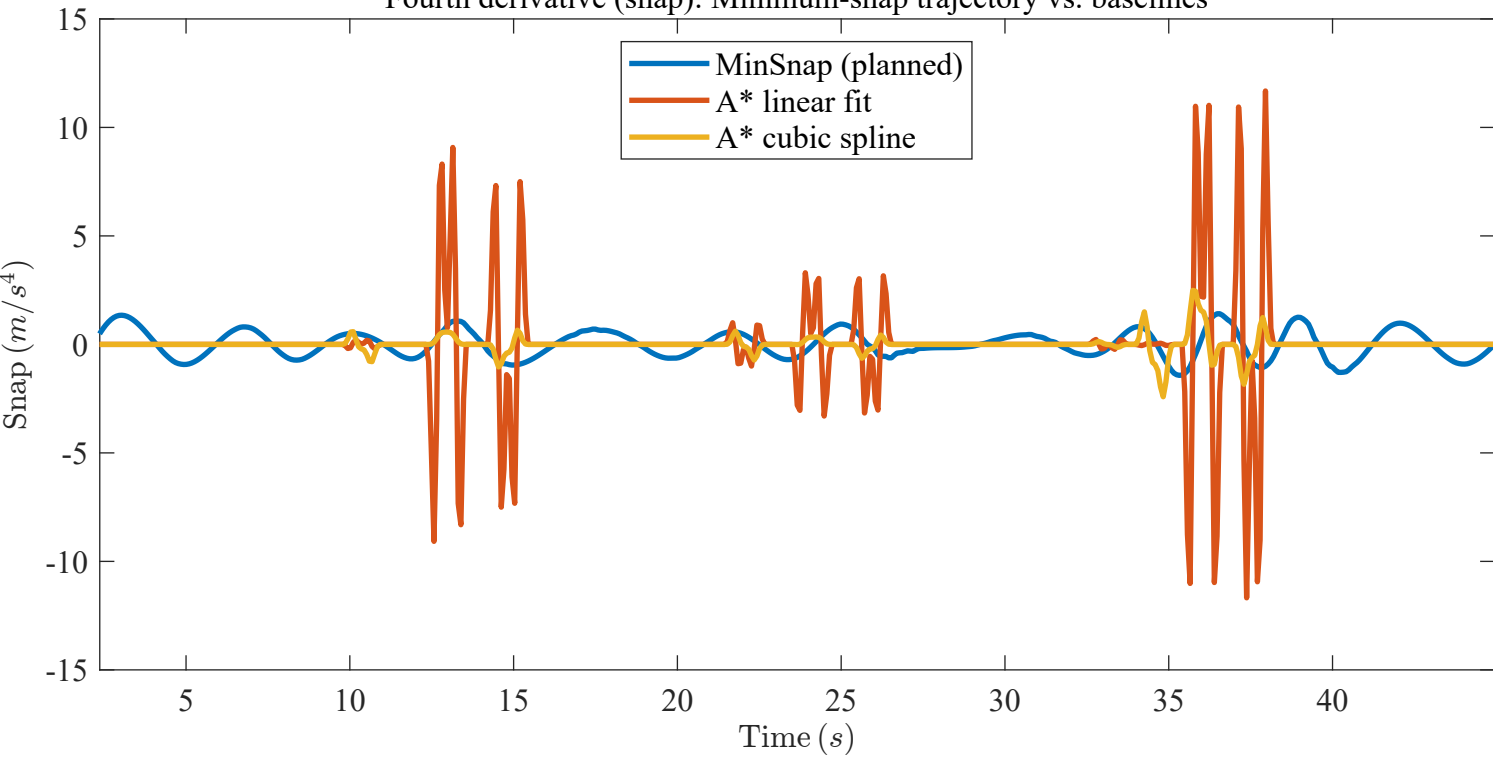
Fourth derivative (snap): Minimum-snap trajectory vs. baselines
