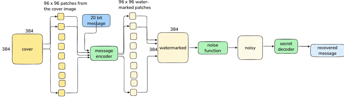
Figure 1: StegoStamp Watermarking and Decoding Architecture. The message encoder refers to F_\theta and the secret decoder refers to D_\phi .
