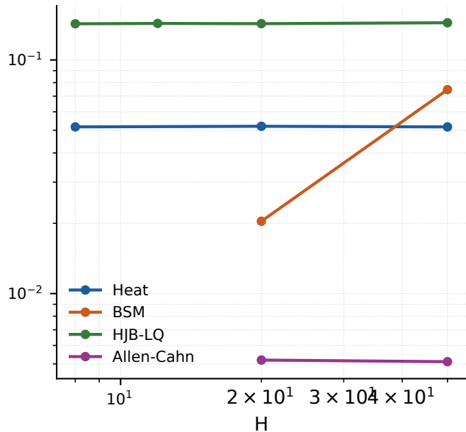
test RMSE
